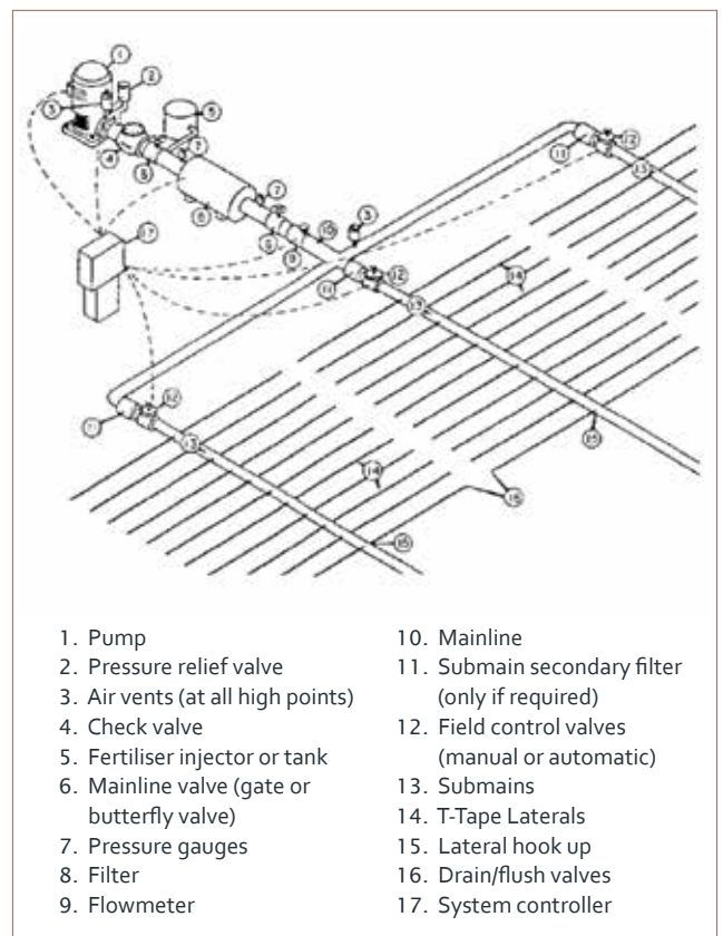
Figure 2: Typical drip system layout.
